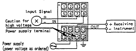
Fig.10 Wiring Diagram
