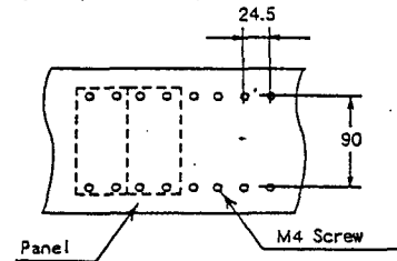
Fig.8 Panel (Wall) Mounting Dimension
